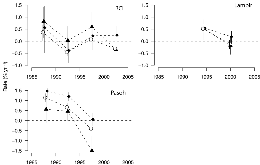
Figure 2. Changes in Aboveground Biomass for Fast- and Slow-Growing Species Groups, BCI, Lambir, and Pasoh, in % y^{-1}
